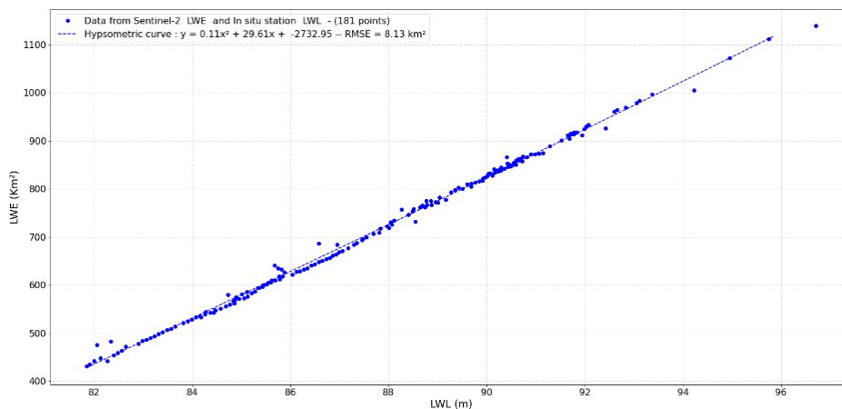
Figure 6 LWE vs LWL in Argyle Lake in Australia with a RMSE of 8.13 km 2 , or uncertainty of 0.73%.
