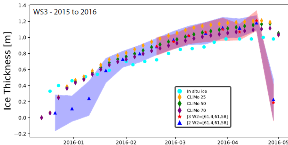
Figure 10 Comparison of LIT estimates over the Great Slave Lake for three winter seasons: 2013-2014 (top), 2014-2015 (middle), and 2015-2016 (bottom). From Mangilli et al. (2022).
