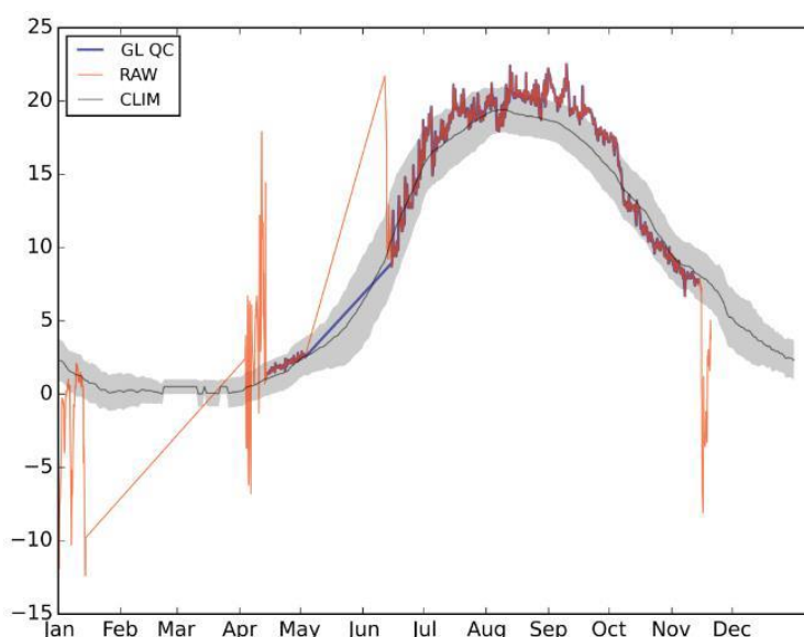
Figure 9 Illustration of quality control results, in this case for Lake Huron in year 2002. The red line is the received in-situ data: when thin, this indicates periods failing quality control, and when thick, data that pass quality control. The black line and grey band show the climatological annual cycle for this location and its inter-annual variability (one sigma).
