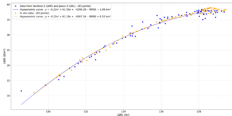
Figure 5 Hypsometric curves computed for Lac de Der (France) with LWE derived from Sentinel-2 time series and LWE from in-situ data (orange dots) and altimetric data, i.e. Jason 3 (blue dots).
