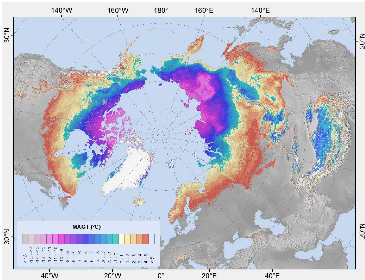
Figure 1: Modelled Mean Annual Ground temperature in regions with permafrost probability larger than zero (GlobPermafrost). Data: Obu et al., 2018, 2019
